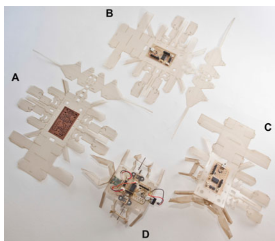
Fig. 5. Overview of the origami-inspired printed robot fabrication process. (a) Mechanical substrate (PEEK) is laser machined to define the crease pattern and the electrical system consisting of a circuit etch mask printed using a commercial solid-ink printer onto a layer of copper is laminated onto the mechanical substrate. (b) Exposed copper is etched away with ferric chloride, and discrete electrical components and actuators are added with pick-and-place assembly. (c) and (d) Design is folded and locked into place with integrated tab-and-slot fasteners.
