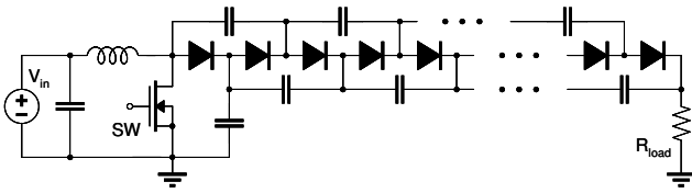
Fig. 7. Hybrid voltage multiplier.
