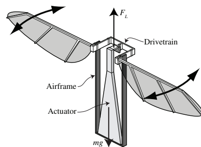
Fig. 1. Illustration of typical Harvard microrobotic fly, similar to the one in [1]. This particular design is described in [13] (drawing courtesy of P. S. Sreetharan).
