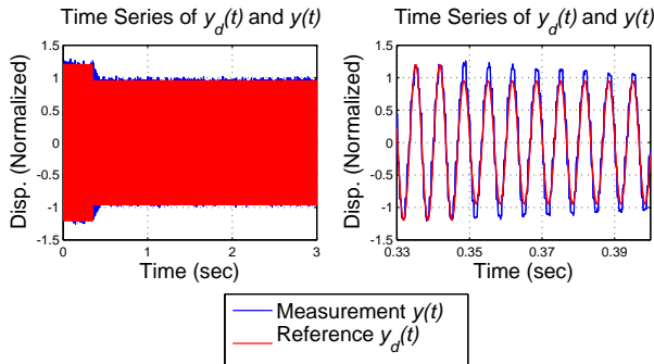
Fig. 16. Comparison of time series y_d(t) and y(t) generating the average lift force in Fig. 15. Left Plot : Complete series. Right Plot : Transition from A_r = 1.2 to A_r = 0.95 .
