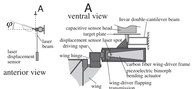
Fig. 2. Diagram of experimental setup used for measuring instantaneous lift forces and displacements of the actuator's tip. The wing-driver is attached to an Invar double-cantilever beam, whose deflection is measured by a capacitive displacement sensor. This deflection is proportional to the lift force, for small deformations of the beam. The displacement of the actuator's tip is measured using a CCD laser displacement sensor. For details on the force sensor see [14].
