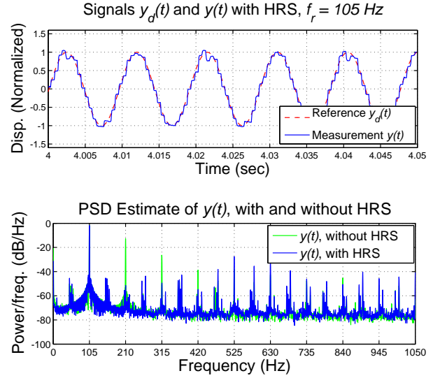
Fig. 9. Case 3. Upper Plot: Time series of y_d(t) = A_r \sin(2\pi f_r t) and y(t) , using the HRS, with A_r = 1 and f_r = 105 Hz. Bottom Plot: Comparison of PSD estimates of the measured outputs y(t) , with and without using the HRS.
