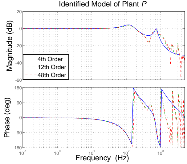
Fig. 4. Bode diagram of identified model \hat{P}(z) of the plant P(z) . A 48th-order model is shown in red, reduced 12th and 4th order models are shown in green and blue, respectively.
