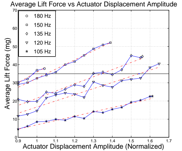
Fig. 12. Empirical relationship between lift force and actuator displacement amplitude, with f_r taking the values 105, 120, 135, 150 and 180 Hz.
